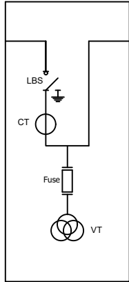
TEK HAT ŞEMASI SINGLE LINE DIAGRAM
